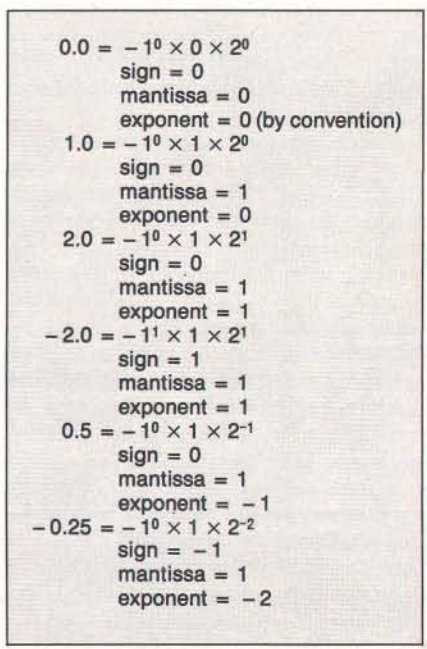
Figure 2: Some common numbers written in the floating-point format.
