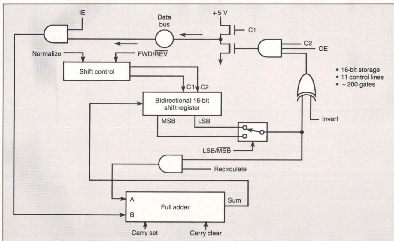
Figure 5: The Accumulator wafer type.
