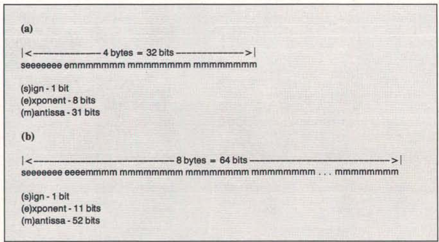
Figure 3: IEEE standard floating-point formats. (a) The format for 4-byte floating-point numbers (float). This representation has a range of \pm 3.4 \times 10^{-38} to \pm 3.4 \times 10^{38} and a precision of six to seven decimal digits. (b) The 8-byte double format, which has a range of \pm 1.7 \times 100^{-308} to \pm 1.7 \times 10^{308} and a precision of 15 to 16 decimal digits.
