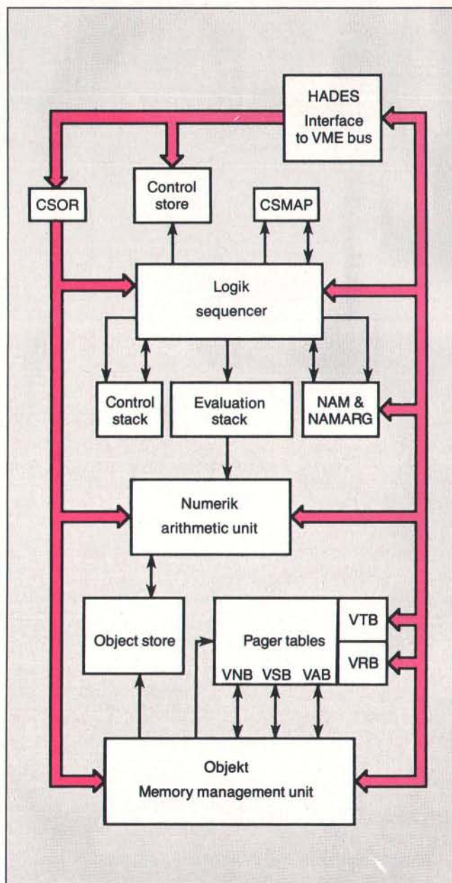
Figure 1: A block diagram of the main functional units of Rekursiv , a persistent-store, object-oriented processor that, in effect, combines the functions of a CPU, memory manager, database manager, and operating system all in one.
