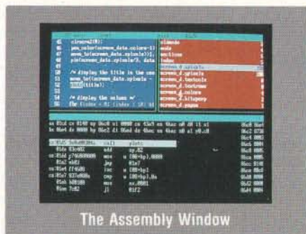
Power Ctrace Debugger
